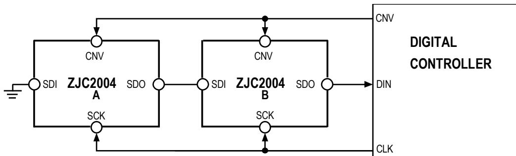
Figure 44. Chain Mode (without Busy Indication) Connection Diagram
