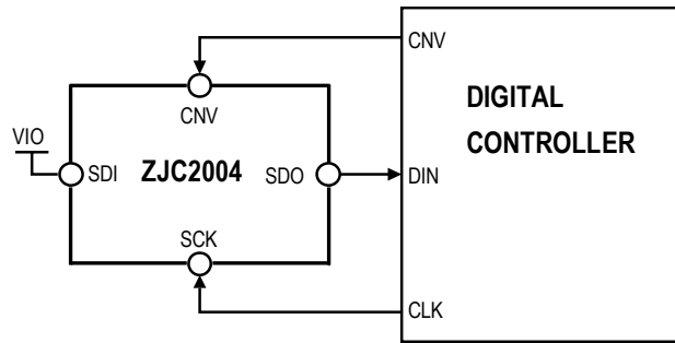
Figure 36. \overline{CS} Mode (3-wire without Busy Indication) Connection Diagram
