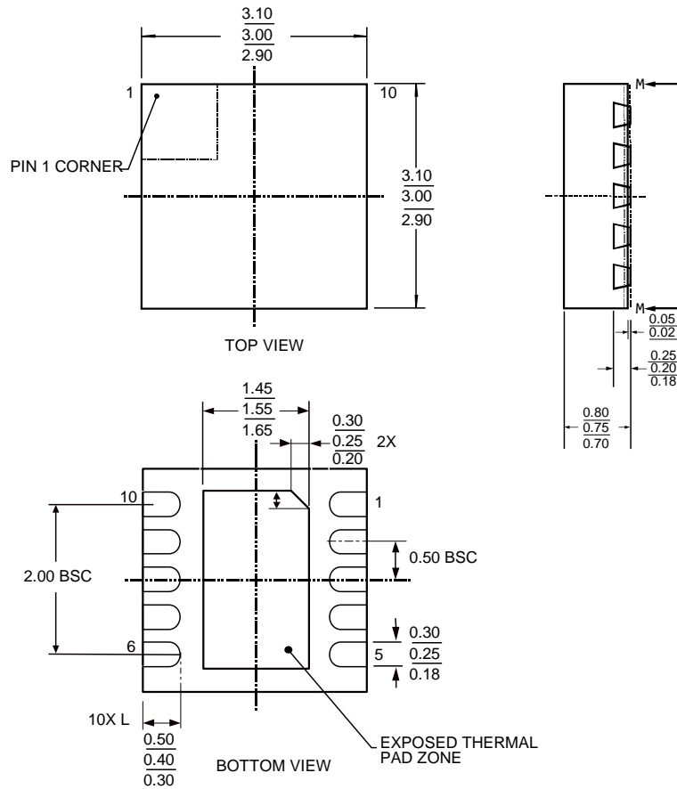
Figure 50. 10-Lead DFN Package Dimensions shown in millimeter
