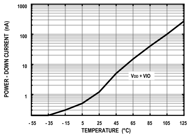
Figure 22. Stand-by Current vs. Temperature
