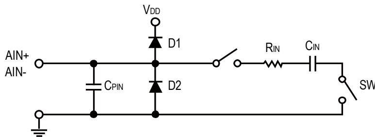
Figure 28. Two Diodes D1 and D2 Provide ESD Protection for the Analog Inputs
