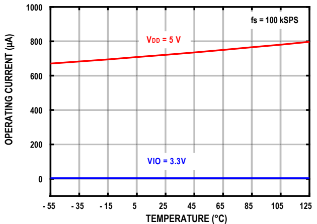
Figure 24. Operating Current vs. Temperature
