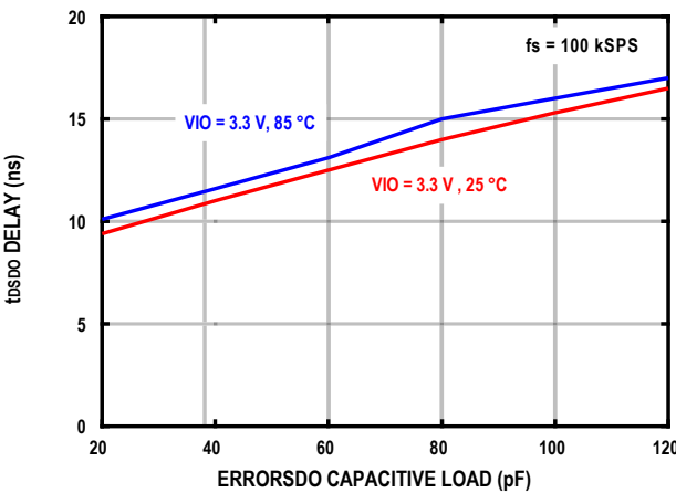
Figure 23. t_{SDO} Delay vs. Capacity Load and Voltage
