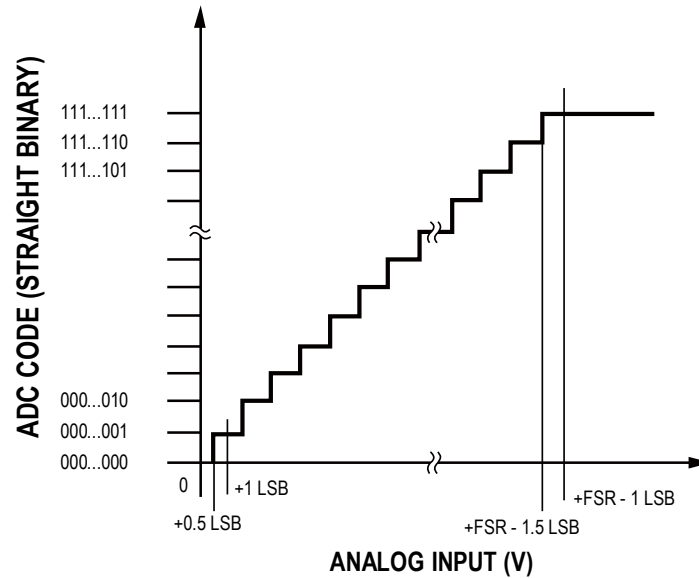
Figure 26. ADC ideal transfer function
