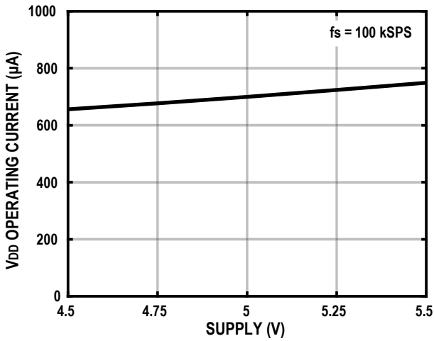
Figure 19. V_{DD} Operating Current vs. Power Supply Voltage
