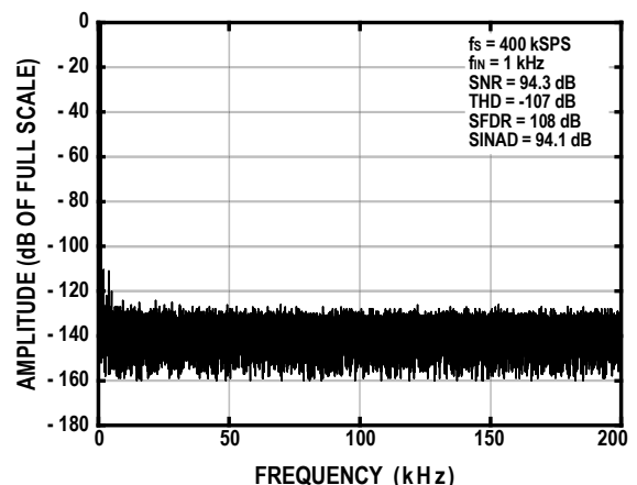
Figure 2. AC Characteristics
