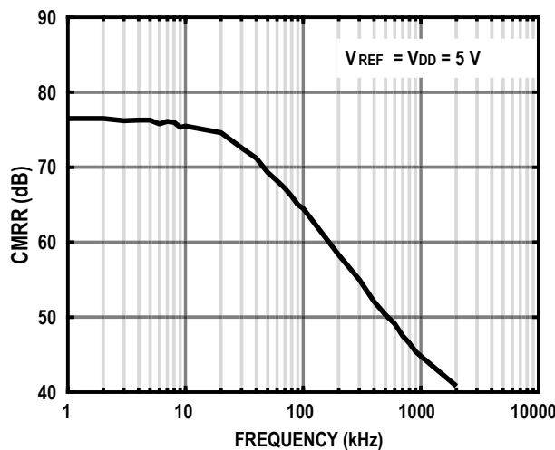
Figure 29. Analog Input CMRR vs. Frequency
