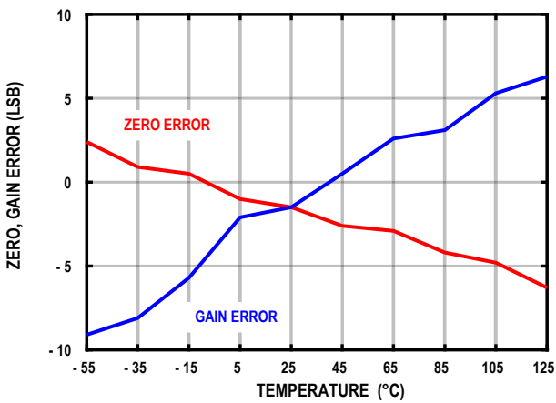
Figure 21. Zero Input, Gain Error vs. Temperature
