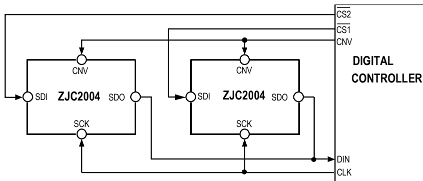
Figure 40. \overline{\text{CS}} Mode (4-wire without Busy Indication) Connection Diagram
