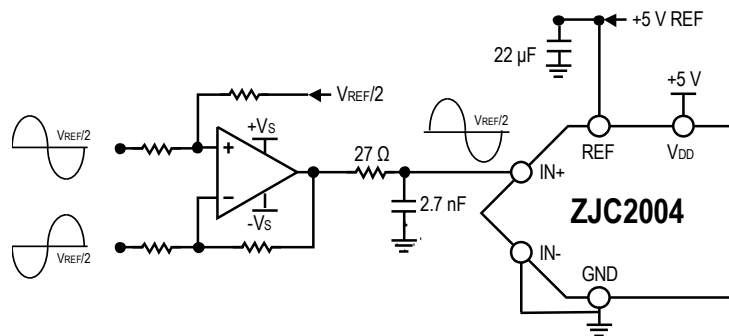
Figure 31. Fully Differential to Single-ended Conversion with an Op Amp
