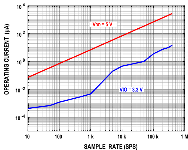
Figure 35. Operating Current vs. Sampling Rate
