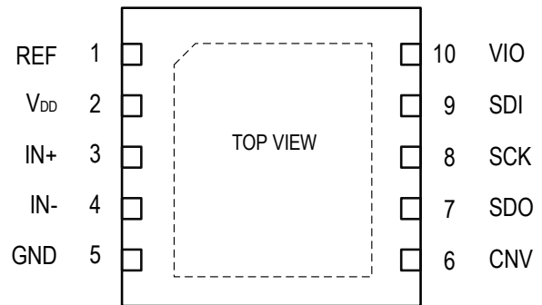
Figure 4. 10-lead DFN pin configuration
