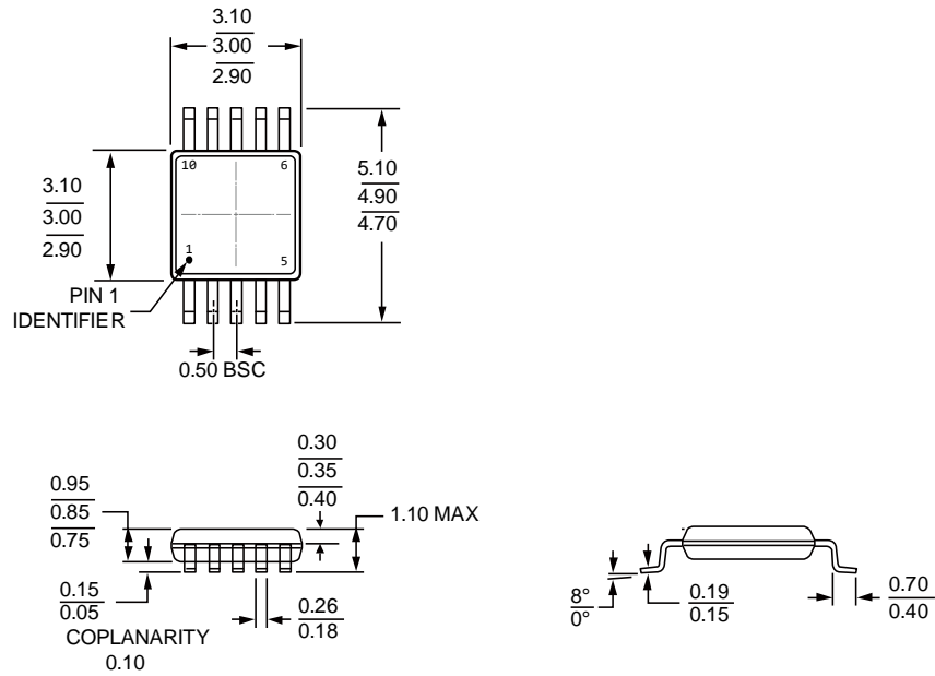
Figure 49. 10-Lead MSOP Package Dimensions shown in millimeter
