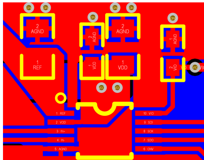
Figure 48. Example Layout and Routing of ZJC2004
