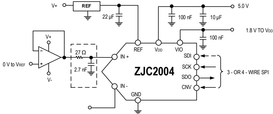
Figure 27. Application Circuits Using Multiple Power Supplies
