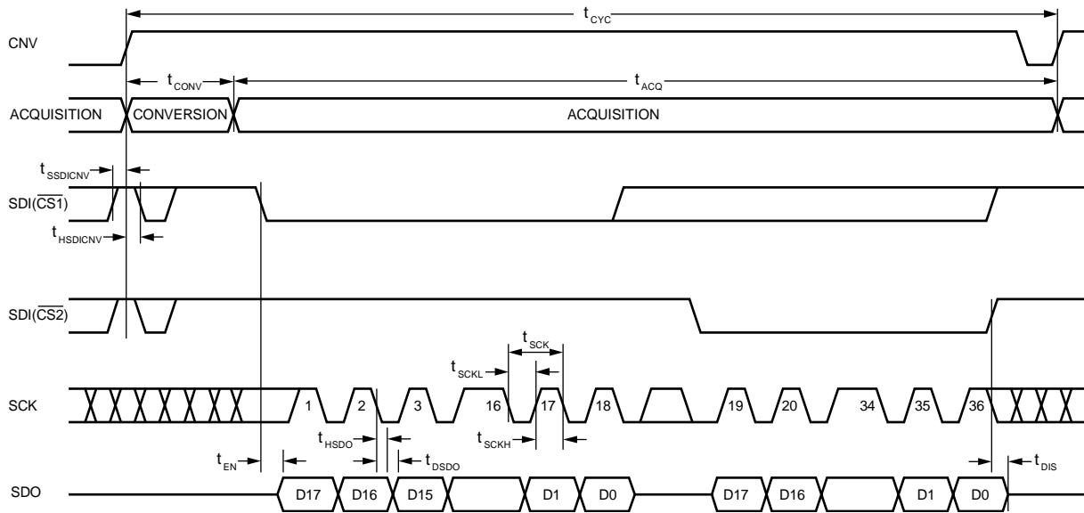
Figure 41. \overline{\text{CS}} Mode (4-Wire without Busy Indication) Serial Interface Timing
