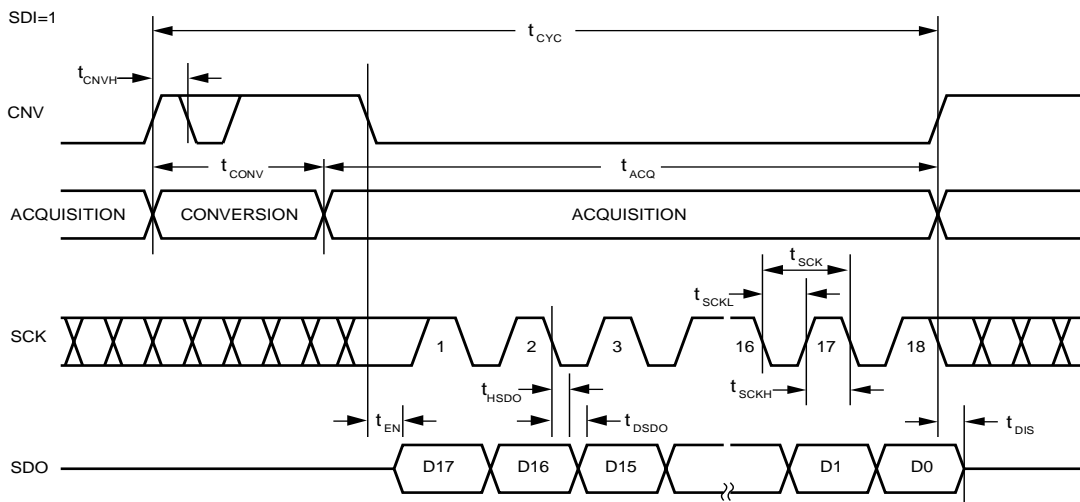
Figure 37. \overline{CS} Mode (3-Wire without Busy Indication) Serial Interface Timing
