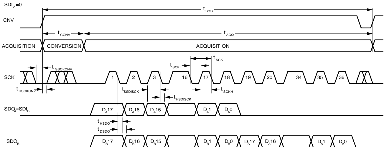
Figure 45. Chain Mode (without Busy Indication) Serial Interface Timing
