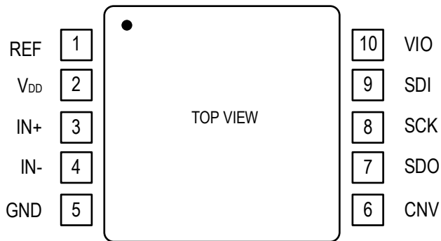
Figure 3. 10-lead MSOP pin configuration
