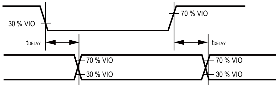
Figure 6. Voltage Levels for Timing
